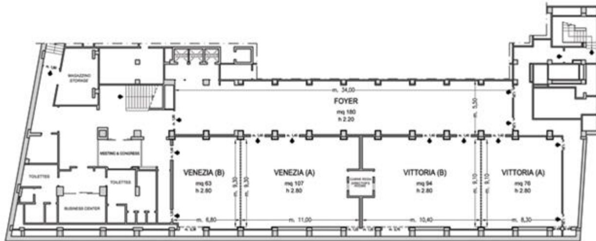
Piano -1 / Basement
